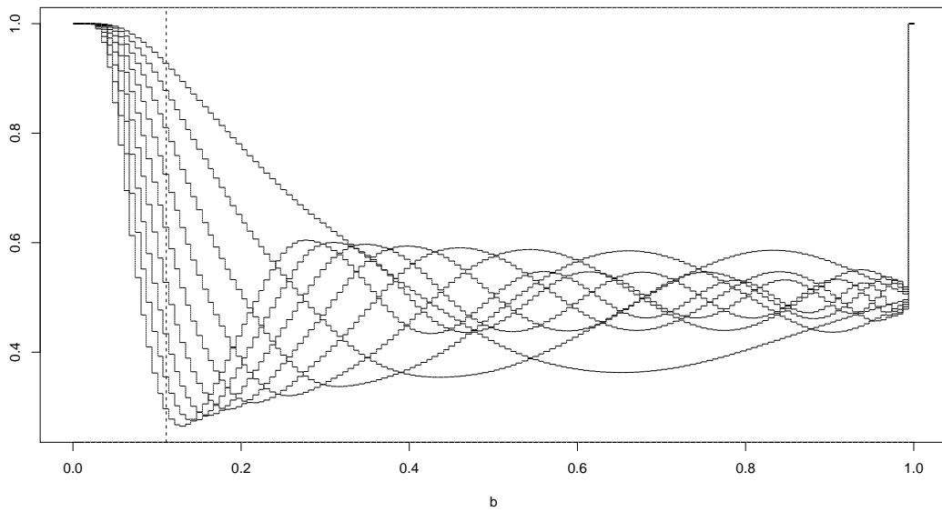
Figure 1: Numerical values of P_{0, I_n}(\hat{\omega}_{\mathcal{W}} \geq 0) for \mathcal{W}_{ij} = \mathbf{1}_{(-1,1)}((i-j)/(bn)) as a function of b . Sample size n = 150 and Assumption 3 holds with k_F = k and for different values of k \in \{2, 3, 4, \dots, 10\} . The probabilities for k = 2 correspond to the function with the largest value at the dashed vertical line, the probabilities for k = 3 correspond to the function with the second largest value at the dashed vertical line, etc.
